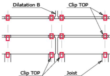
Picture 5 - Butting deck boards with STANDARD clip TOP.
